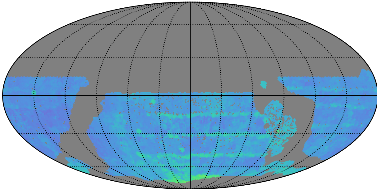
roman_v3.3_10yrs WFD i band: 80thPercentile Season Length
