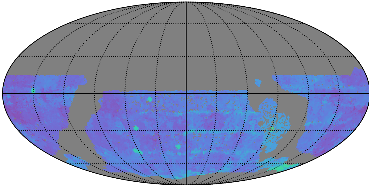
roman_v3.3_10yrs WFD g band: 80thPercentile Season Length
