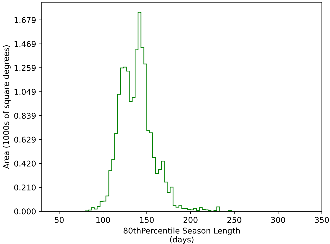
roman_v3.3_10yrs WFD g band: 80thPercentile Season Length
