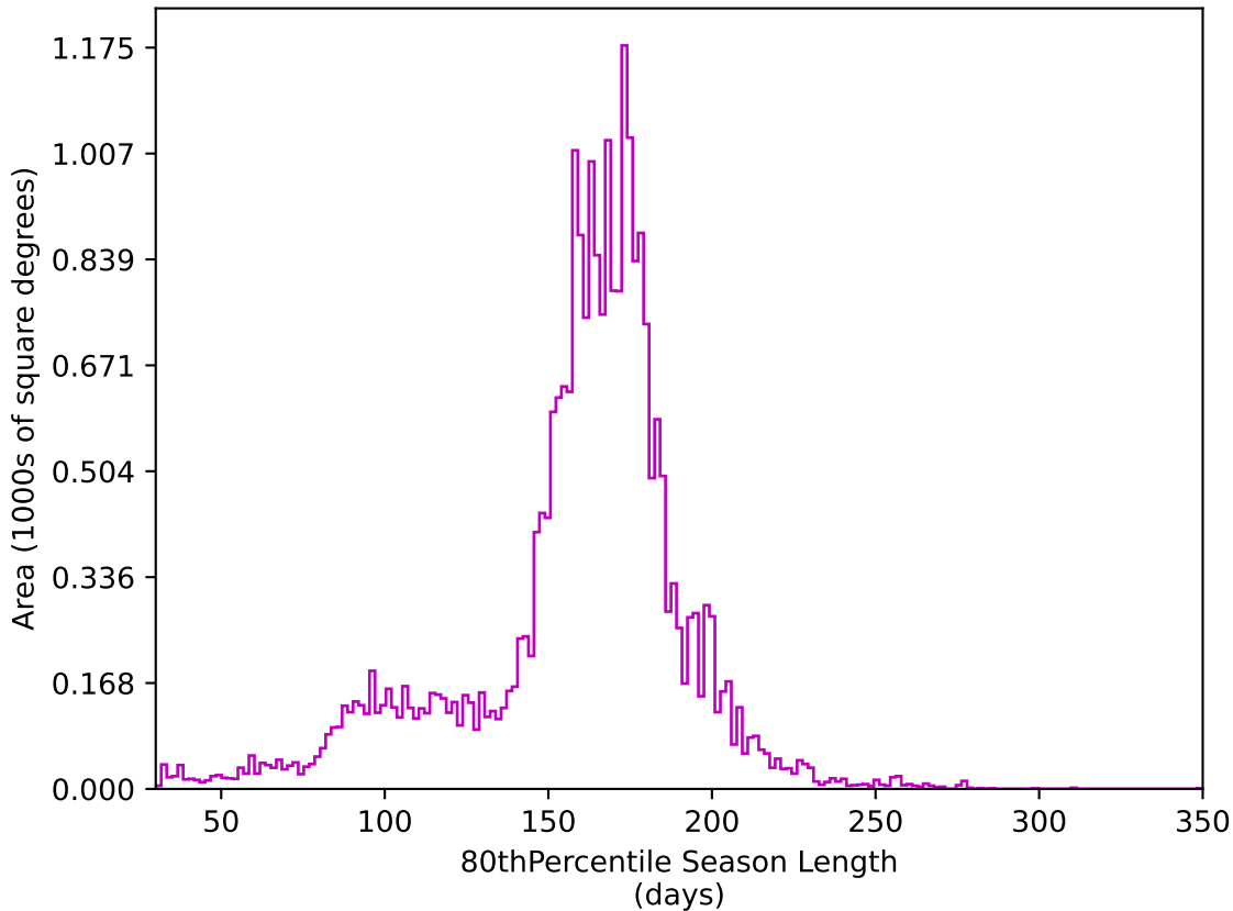
roman_v3.3_10yrs All sky z band: 80thPercentile Season Length
