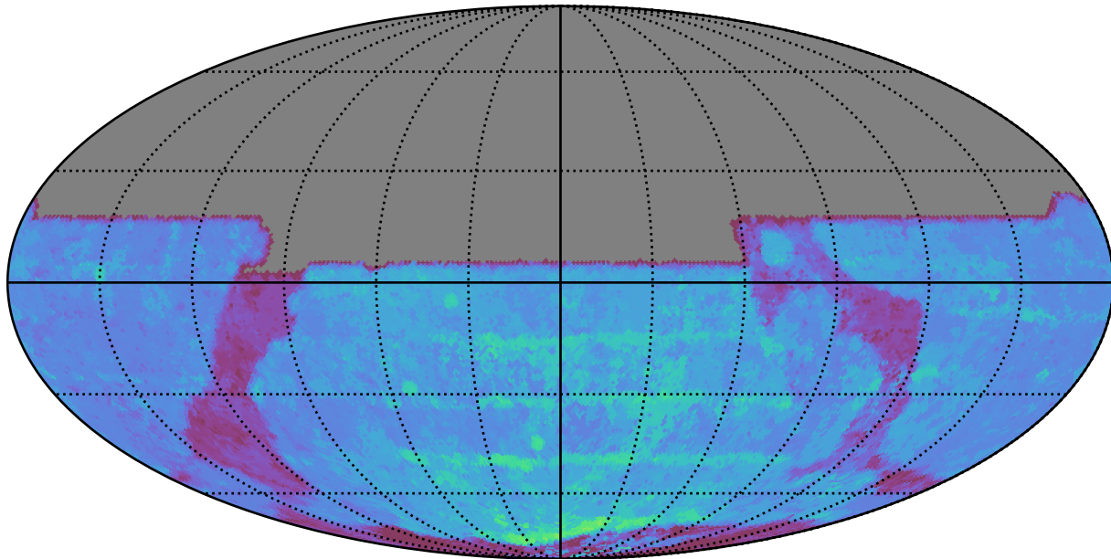
roman_v3.3_10yrs All sky y band: 80thPercentile Season Length
