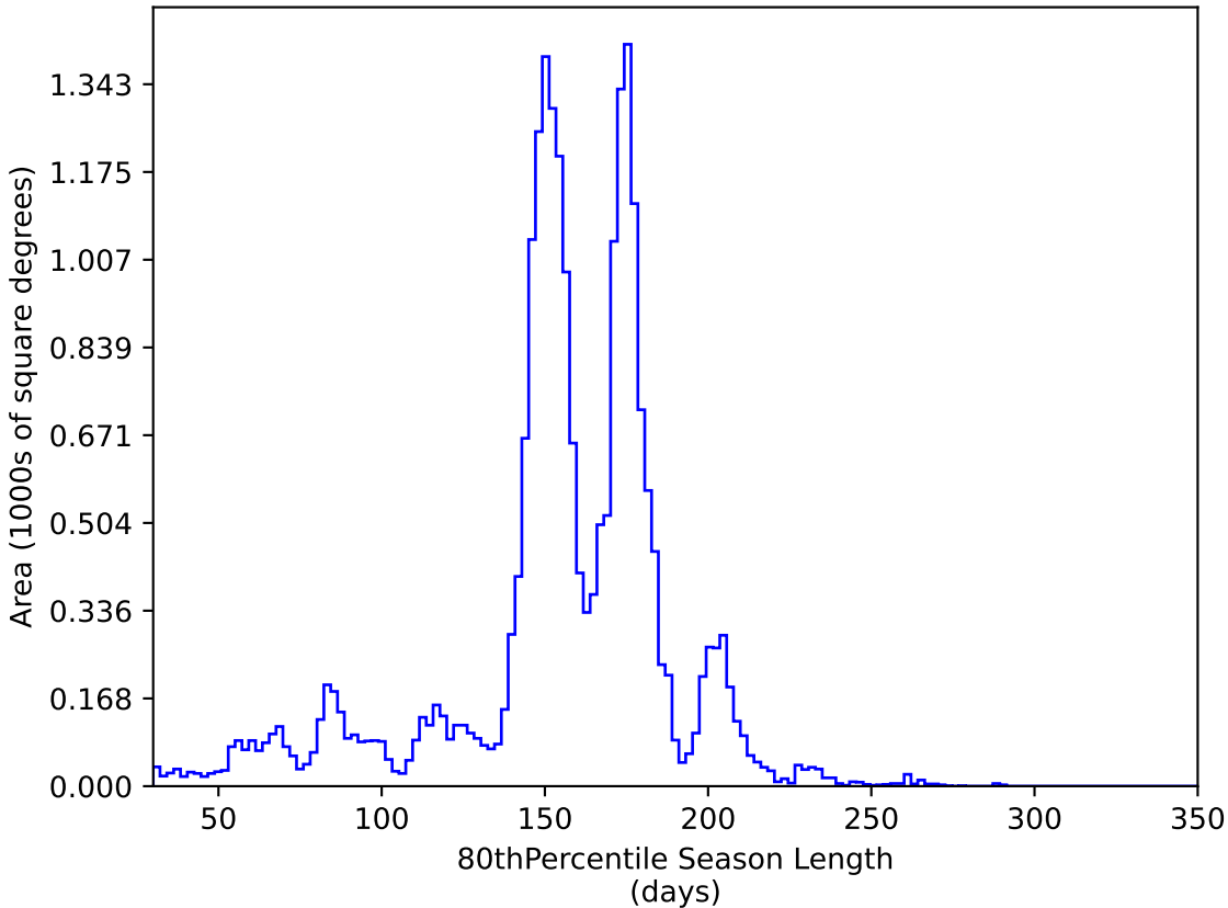
roman_v3.3_10yrs All sky y band: 80thPercentile Season Length
