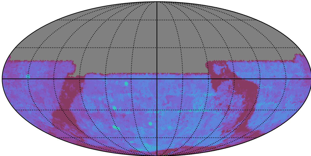
roman_v3.3_10yrs All sky u band: 80thPercentile Season Length
