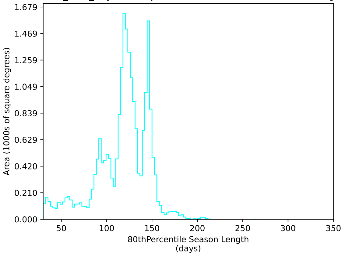
roman_v3.3_10yrs All sky u band: 80thPercentile Season Length
