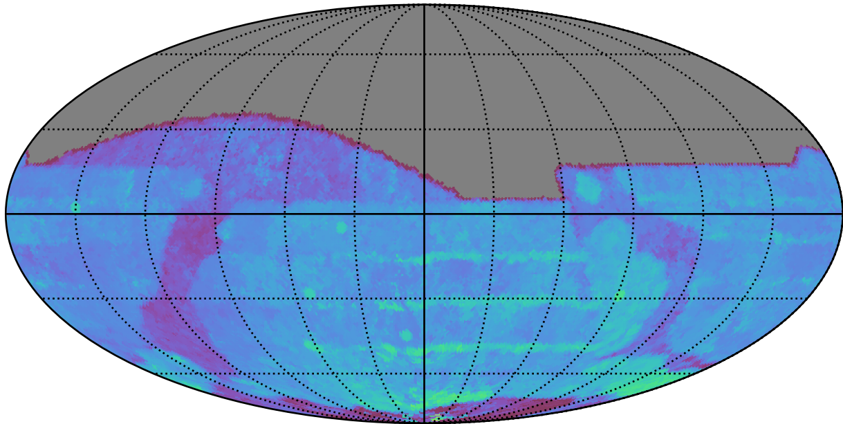
roman_v3.3_10yrs All sky r band: 80thPercentile Season Length
