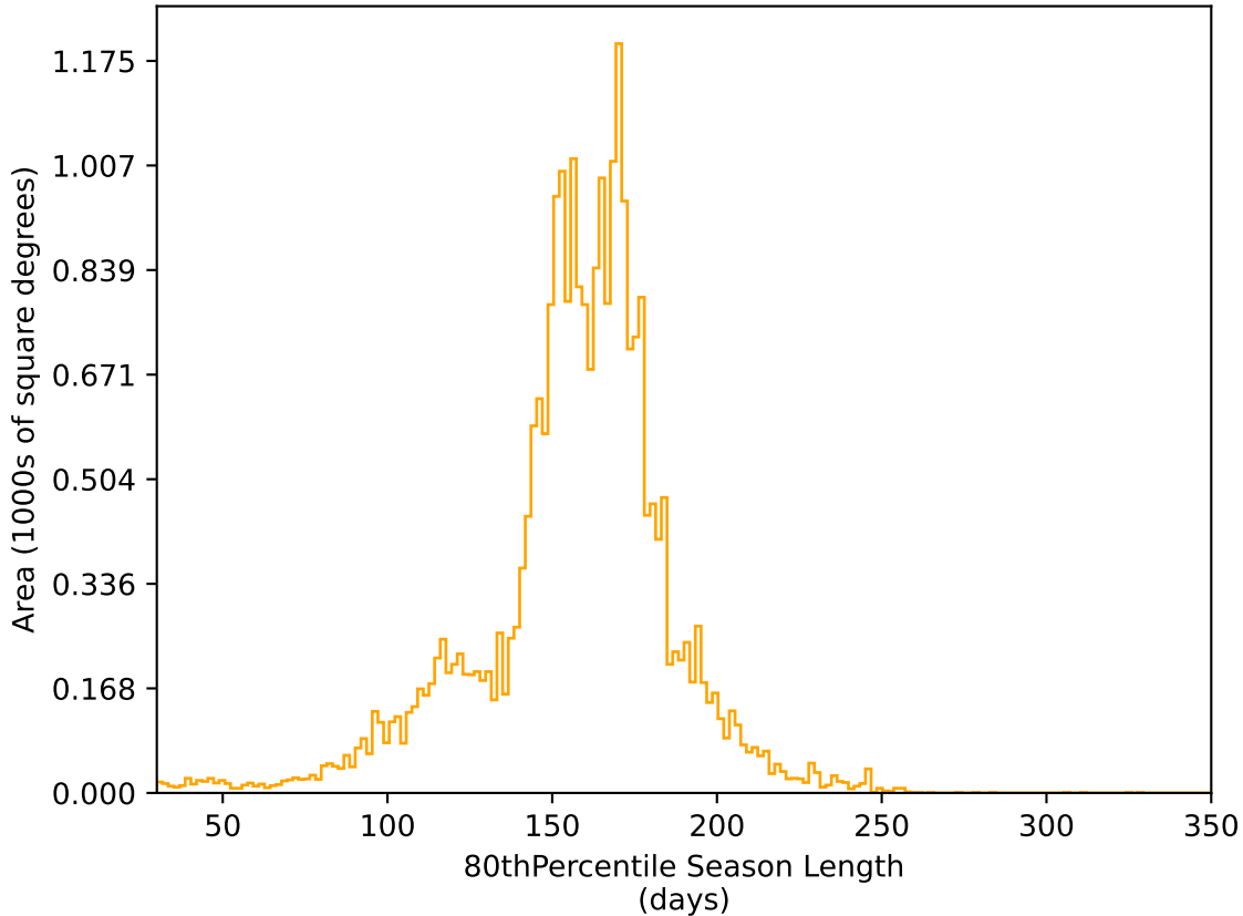
roman_v3.3_10yrs All sky r band: 80thPercentile Season Length
