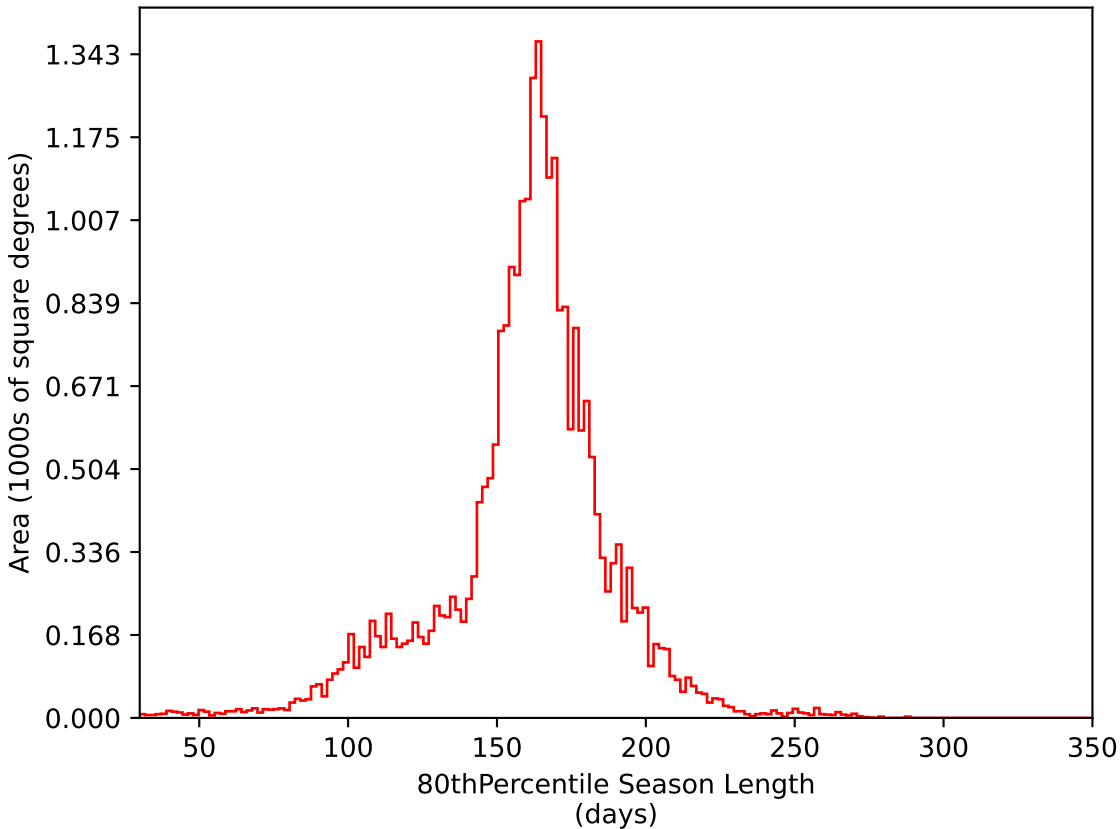
roman_v3.3_10yrs All sky i band: 80thPercentile Season Length
