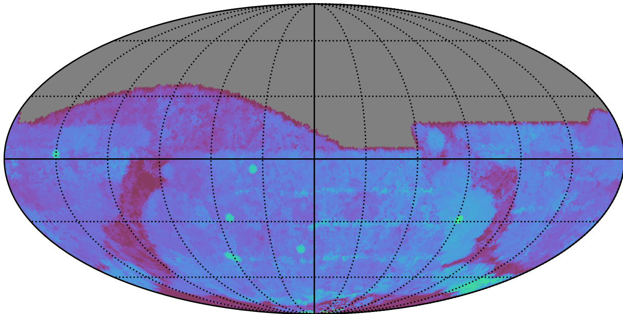
roman_v3.3_10yrs All sky g band: 80thPercentile Season Length
