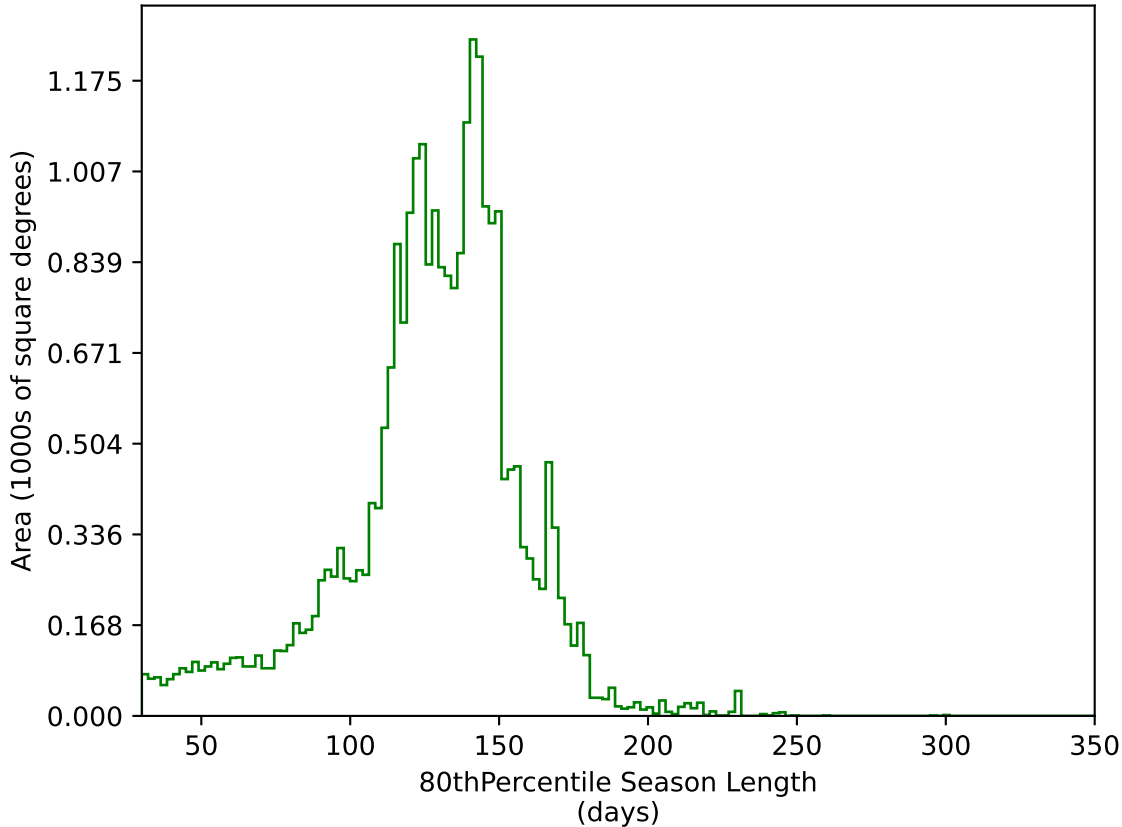
roman_v3.3_10yrs All sky g band: 80thPercentile Season Length
