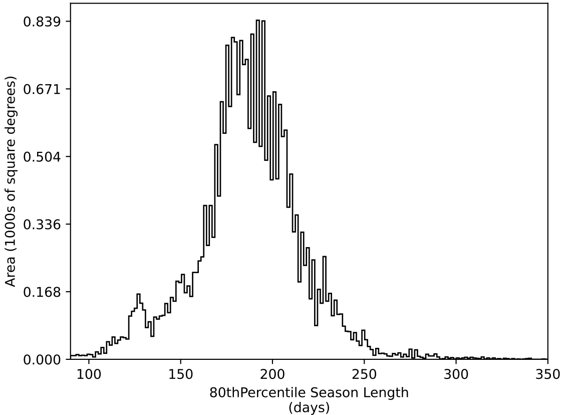
roman_v3.3_10yrs All sky all bands: 80thPercentile Season Length
