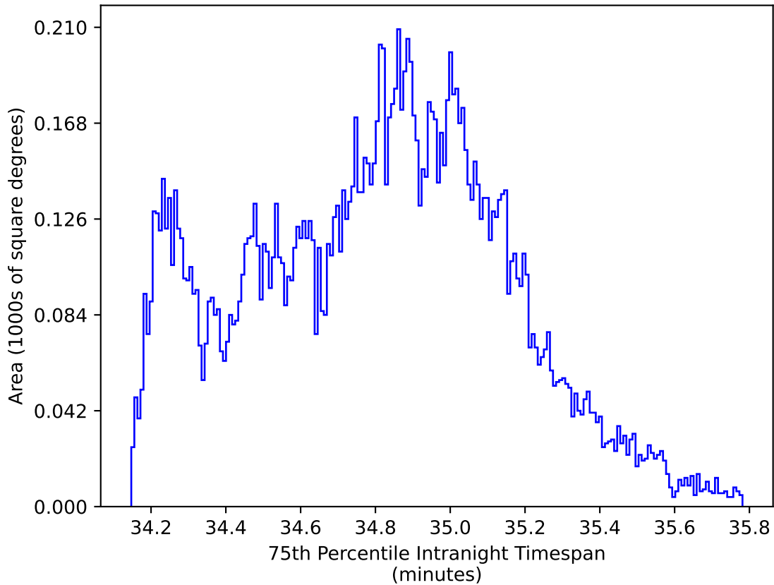
roman_v3.3_10yrs WFD zy bands: 75th Percentile Intranight Timespan
