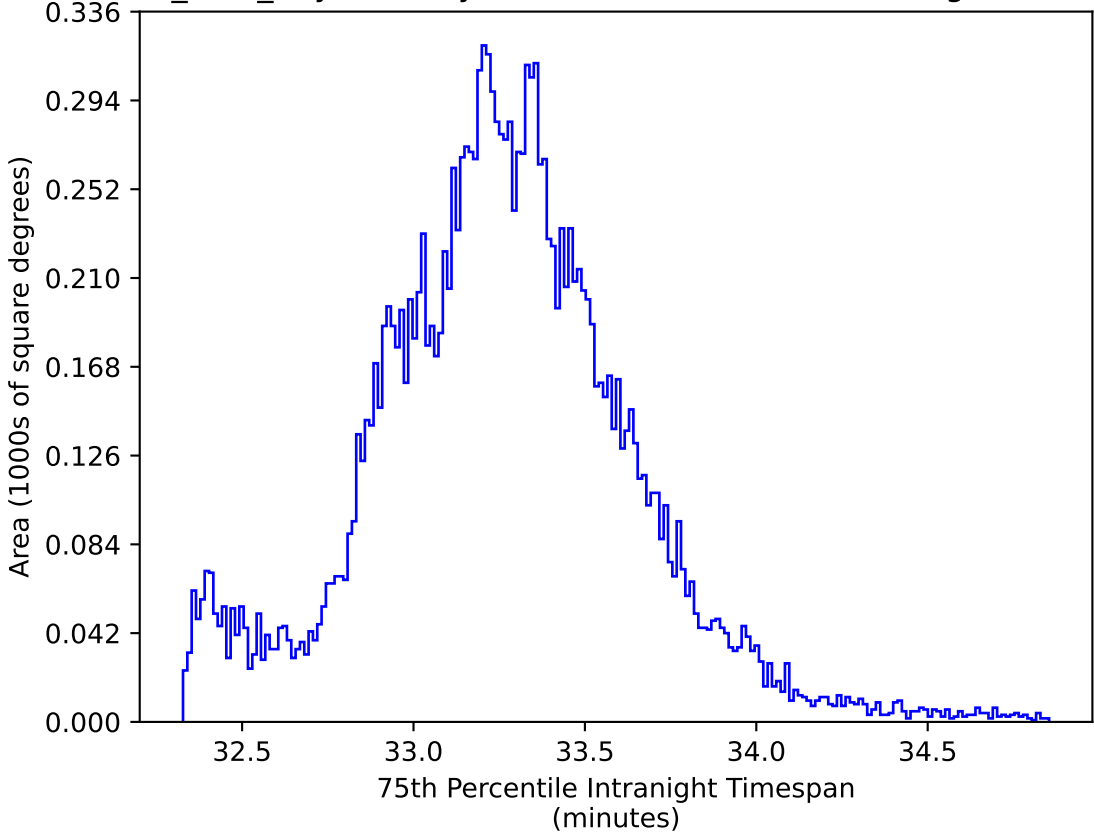
roman_v3.3_10yrs WFD y band: 75th Percentile Intranight Timespan
