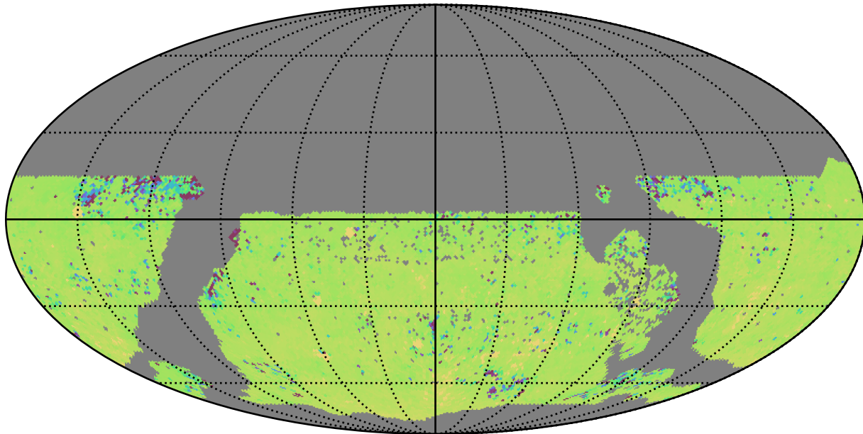
roman_v3.3_10yrs WFD ug bands: 75th Percentile Intranight Timespan
