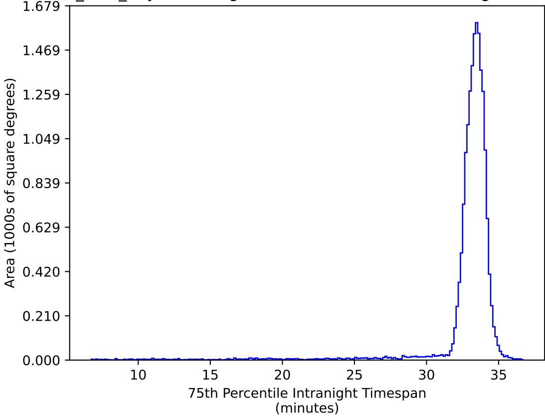
roman_v3.3_10yrs WFD ug bands: 75th Percentile Intranight Timespan
