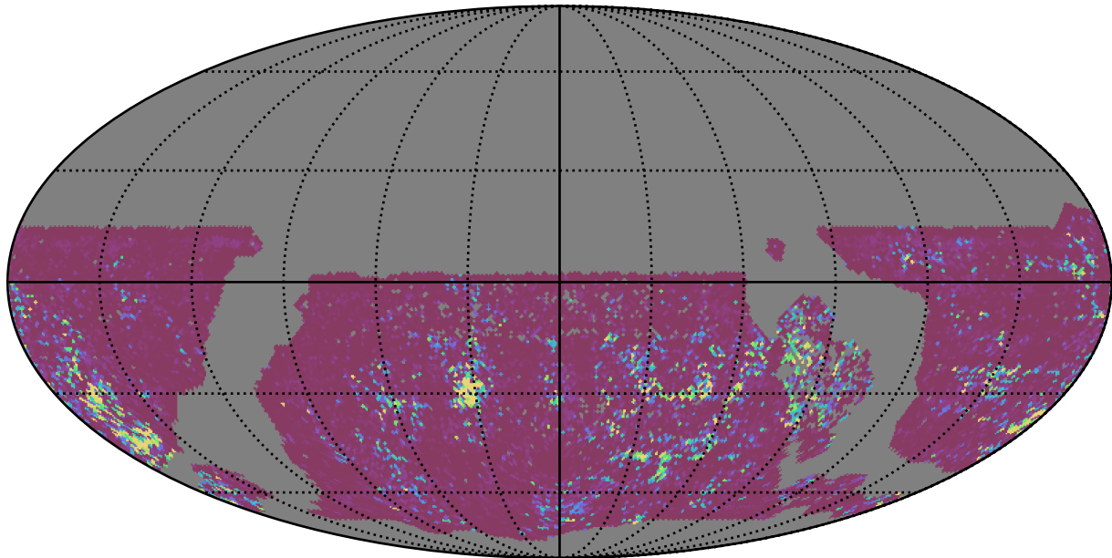
roman_v3.3_10yrs WFD u band: 75th Percentile Intranight Timespan
