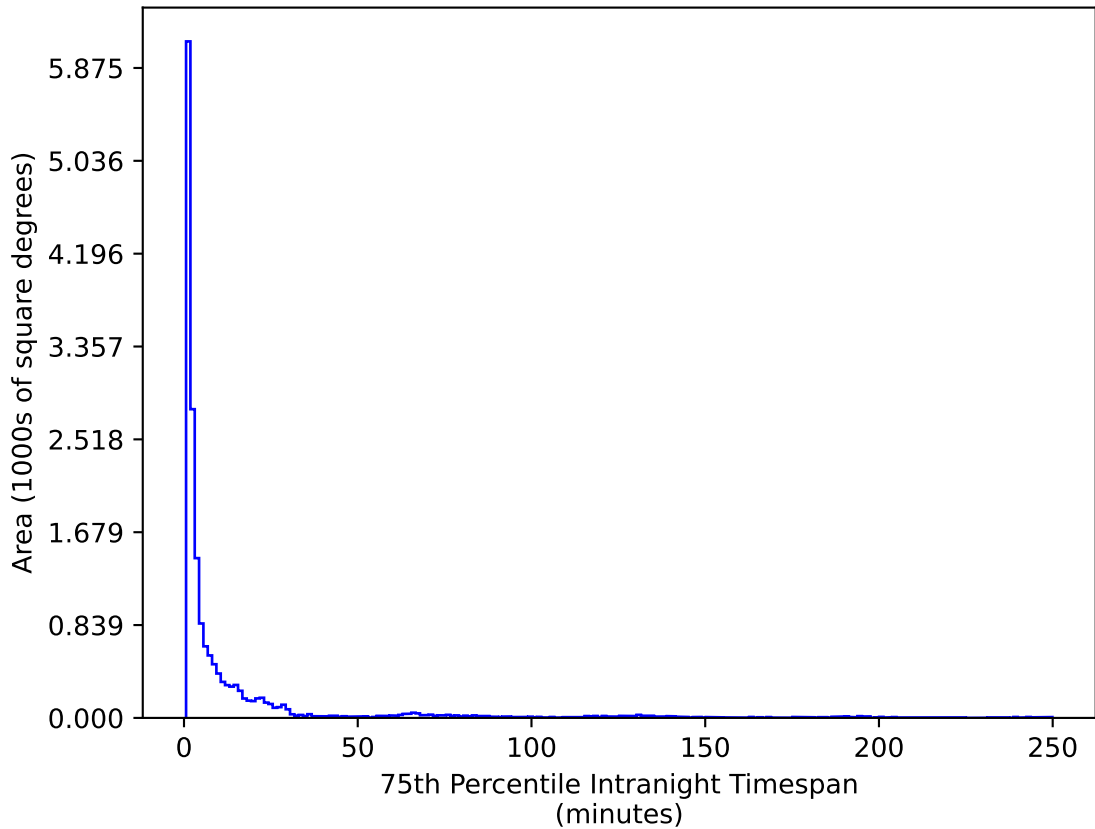
roman_v3.3_10yrs WFD u band: 75th Percentile Intranight Timespan
