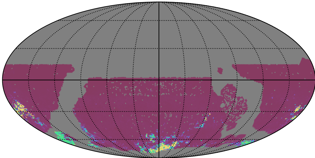
roman_v3.3_10yrs WFD ri bands: 75th Percentile Intranight Timespan
