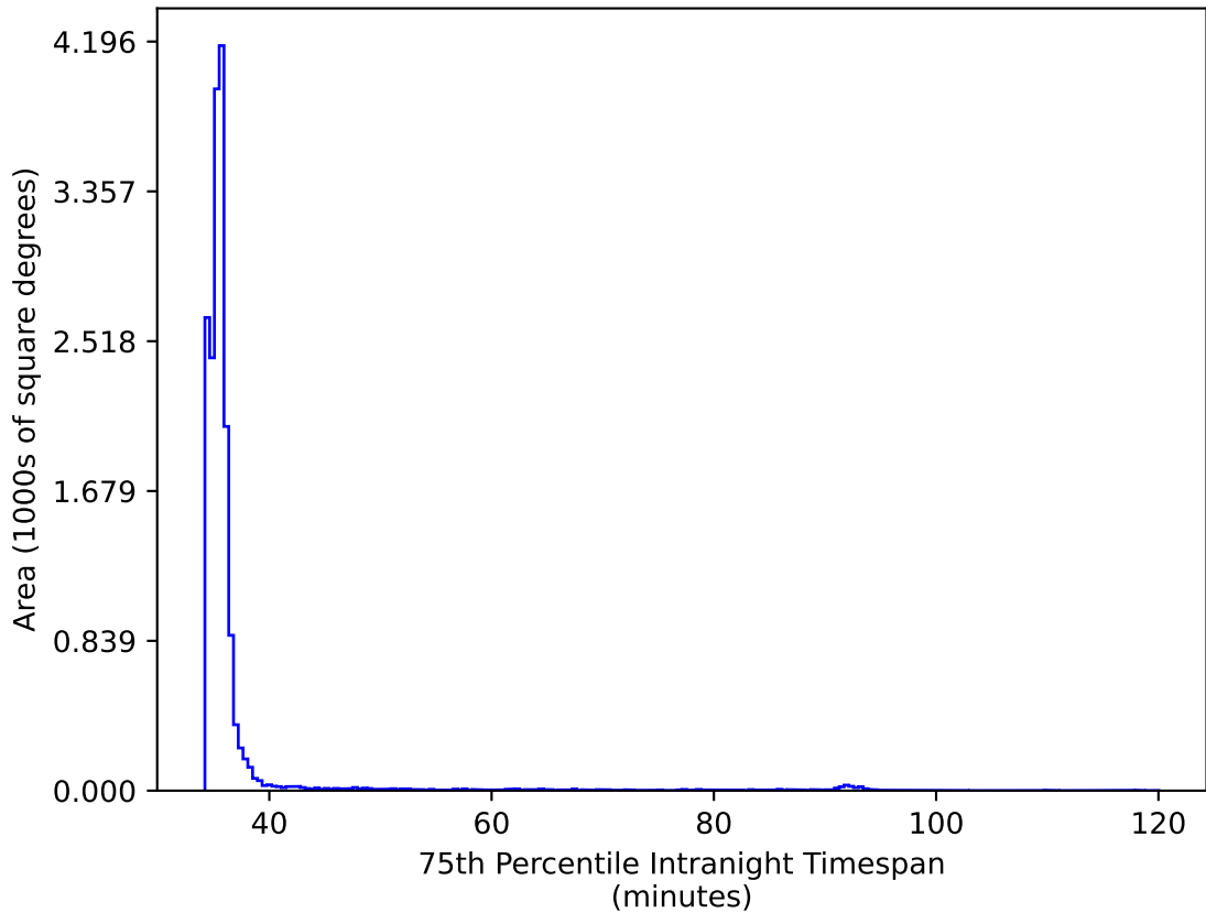
roman_v3.3_10yrs WFD ri bands: 75th Percentile Intranight Timespan
