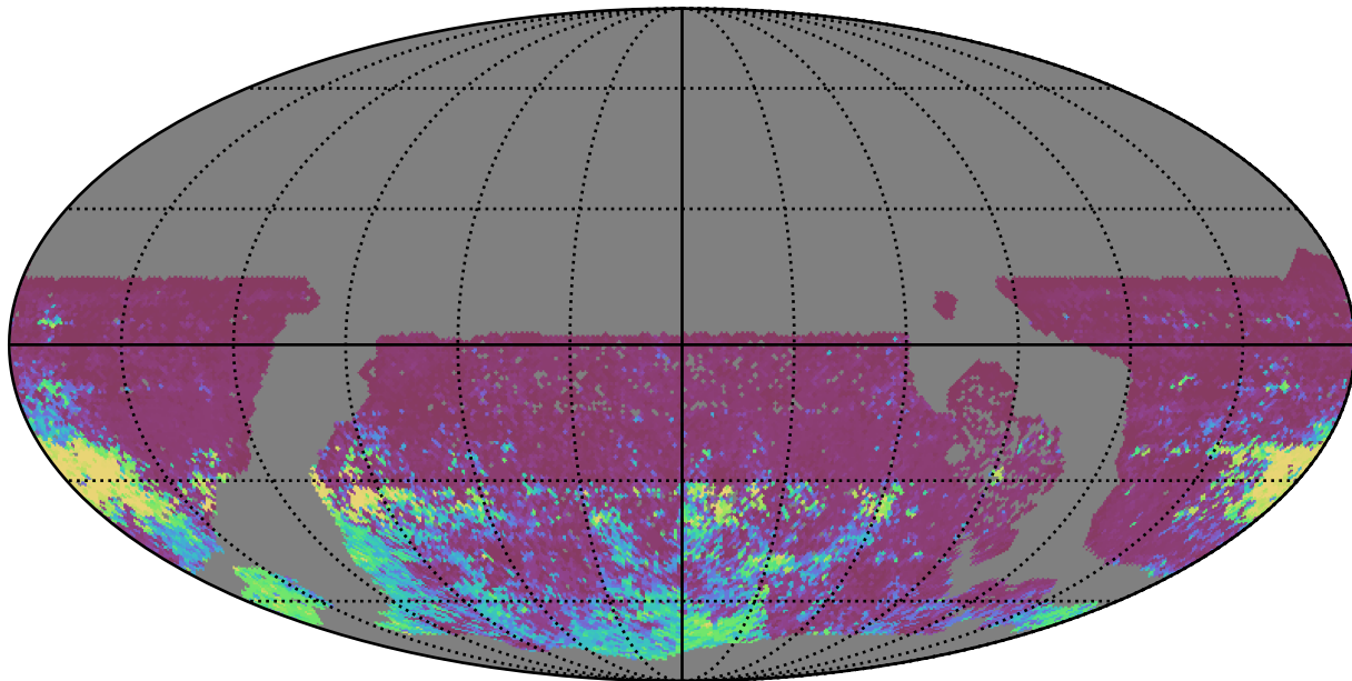
roman_v3.3_10yrs WFD r band: 75th Percentile Intranight Timespan
