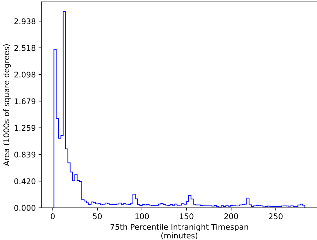
roman_v3.3_10yrs WFD r band: 75th Percentile Intranight Timespan
