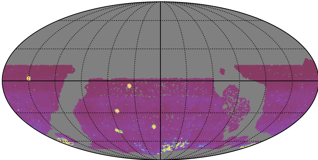
roman_v3.3_10yrs WFD iz bands: 75th Percentile Intranight Timespan
