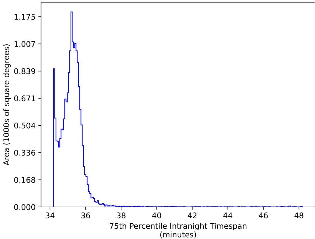
roman_v3.3_10yrs WFD iz bands: 75th Percentile Intranight Timespan
