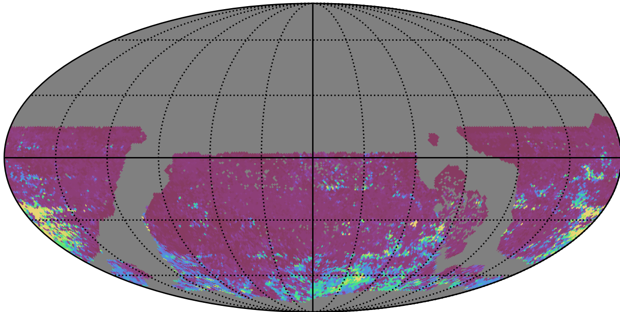
roman_v3.3_10yrs WFD i band: 75th Percentile Intranight Timespan
