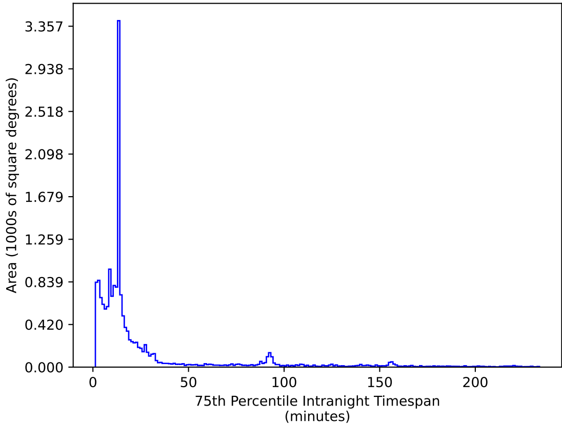
roman_v3.3_10yrs WFD i band: 75th Percentile Intranight Timespan
