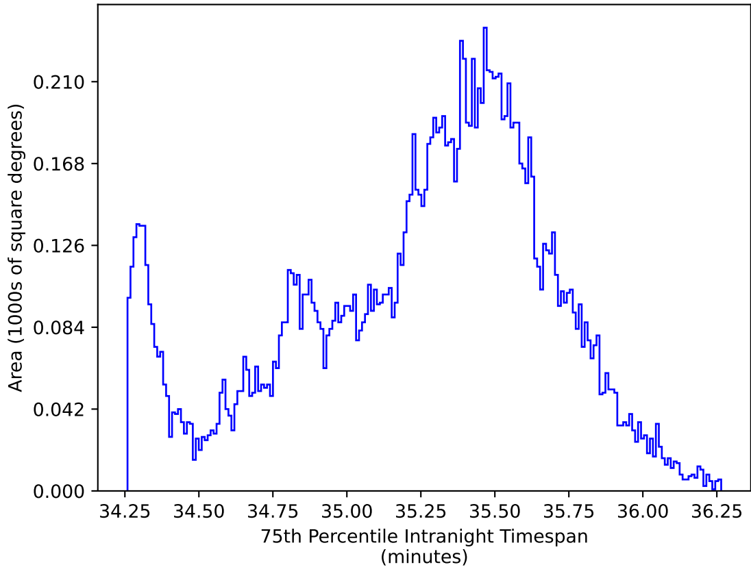
roman_v3.3_10yrs WFD all bands: 75th Percentile Intranight Timespan
