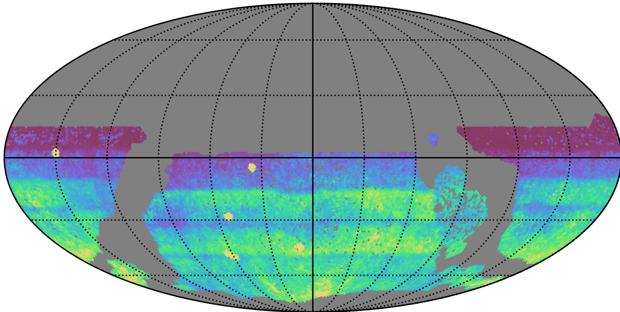
roman_v3.3_10yrs WFD: 75th Percentile Intranight Timespan
