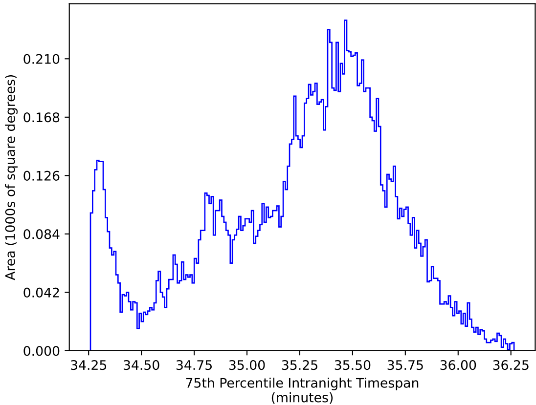
roman_v3.3_10yrs WFD: 75th Percentile Intranight Timespan
