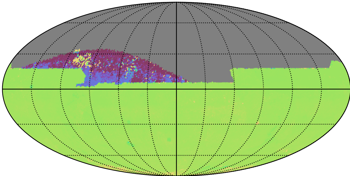
roman_v3.3_10yrs All sky zy bands: 75th Percentile Intranight Timespan
