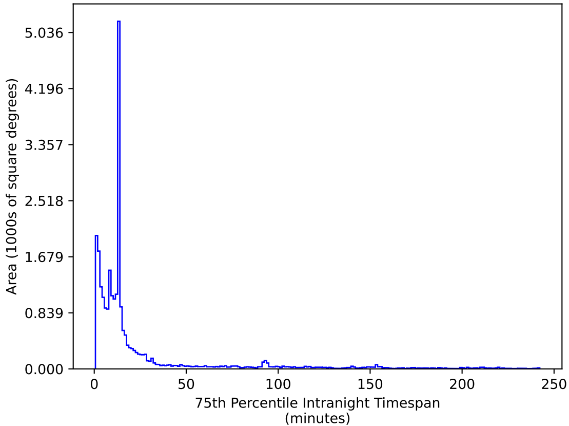
roman_v3.3_10yrs All sky z band: 75th Percentile Intranight Timespan
