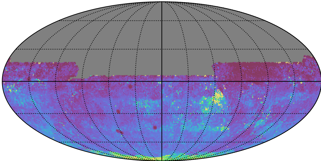
roman_v3.3_10yrs All sky y band: 75th Percentile Intranight Timespan
