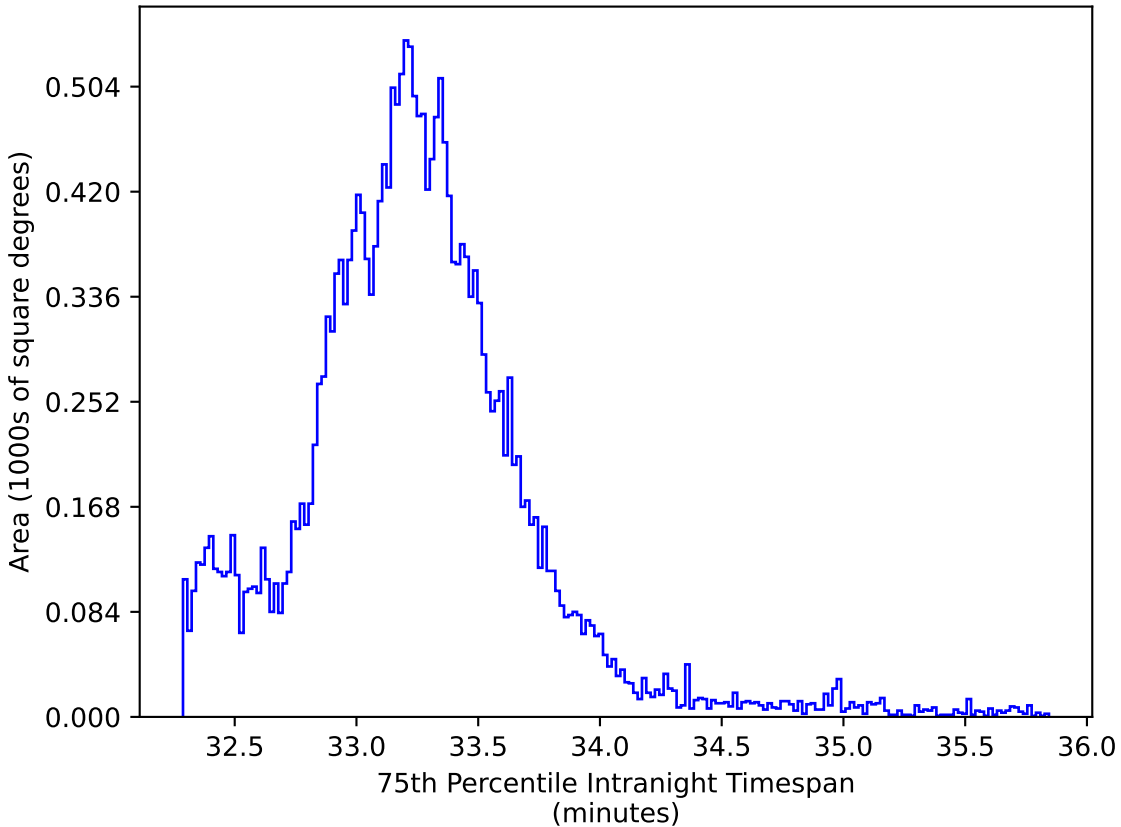
roman_v3.3_10yrs All sky y band: 75th Percentile Intranight Timespan
