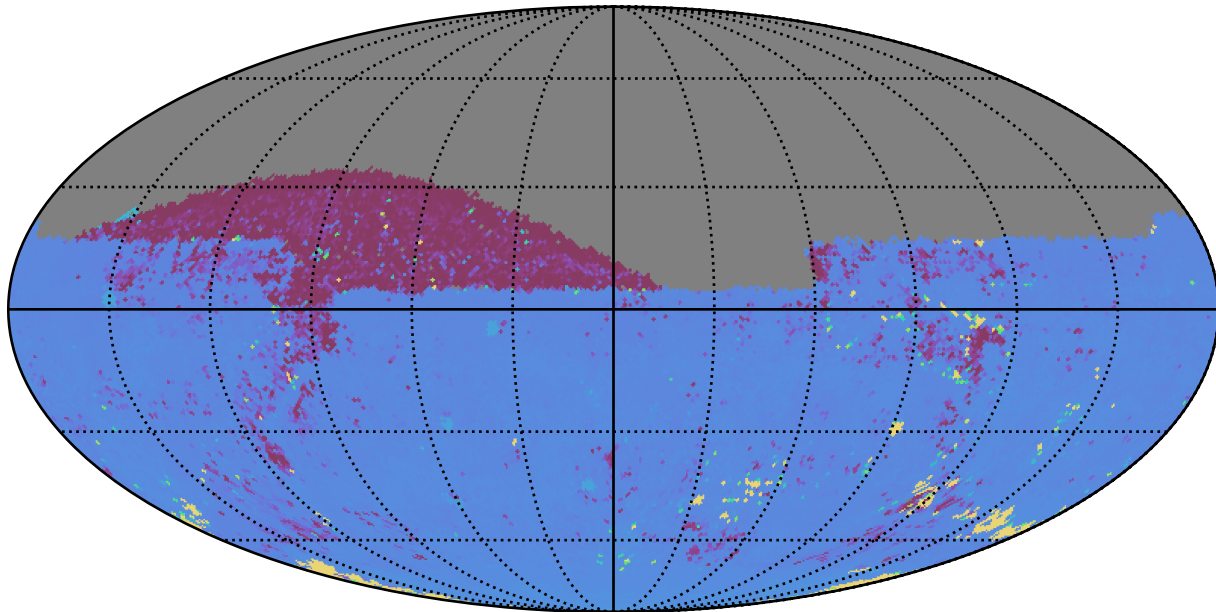
roman_v3.3_10yrs All sky ug bands: 75th Percentile Intranight Timespan
