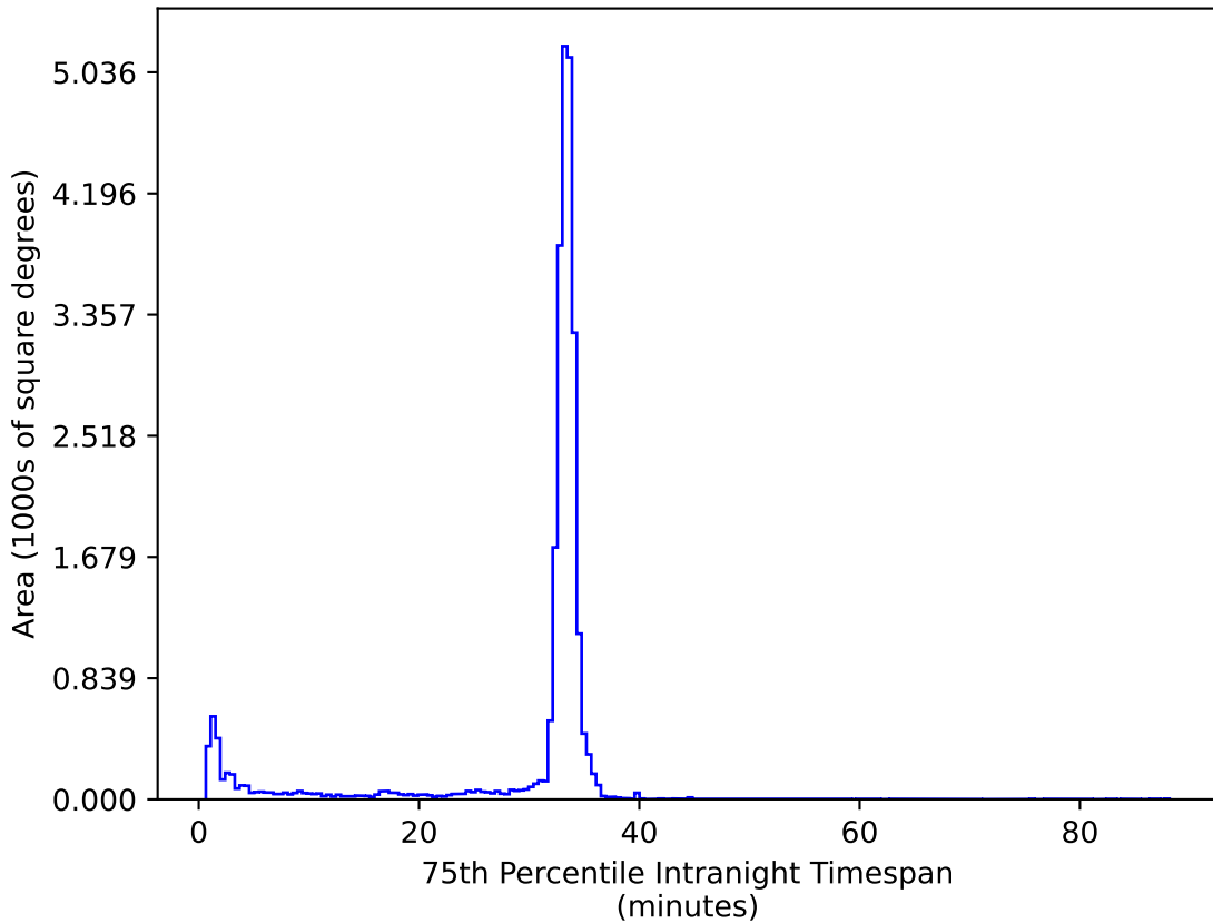
roman_v3.3_10yrs All sky ug bands: 75th Percentile Intranight Timespan
