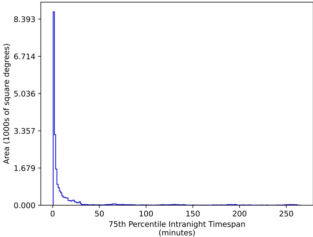
roman_v3.3_10yrs All sky u band: 75th Percentile Intranight Timespan
