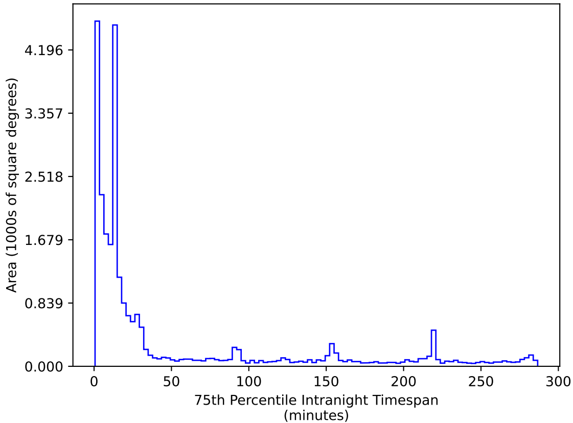
roman_v3.3_10yrs All sky r band: 75th Percentile Intranight Timespan
