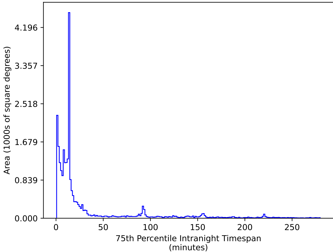
roman_v3.3_10yrs All sky i band: 75th Percentile Intranight Timespan
