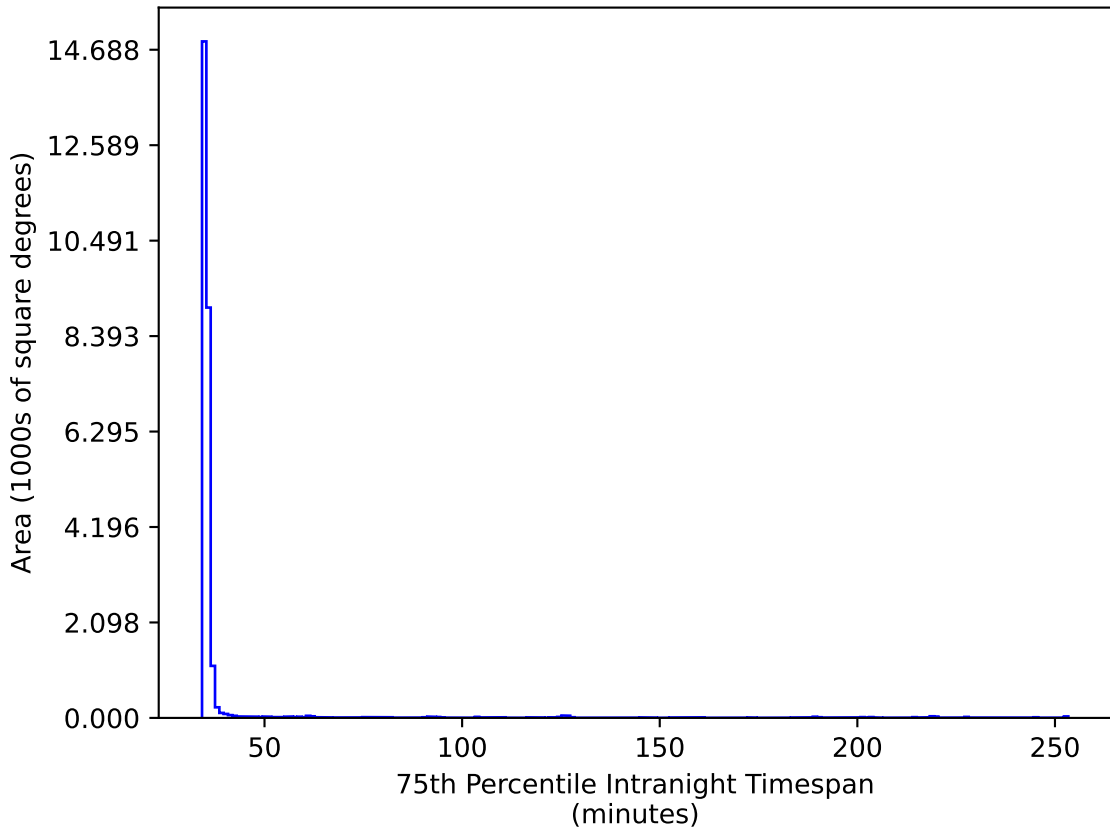
roman_v3.3_10yrs All sky gr bands: 75th Percentile Intranight Timespan
