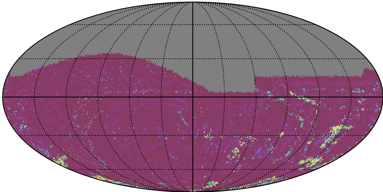
roman_v3.3_10yrs All sky g band: 75th Percentile Intranight Timespan
