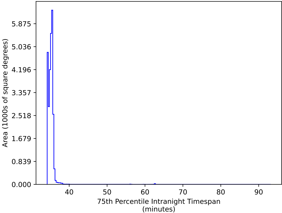
roman_v3.3_10yrs All sky: 75th Percentile Intranight Timespan
