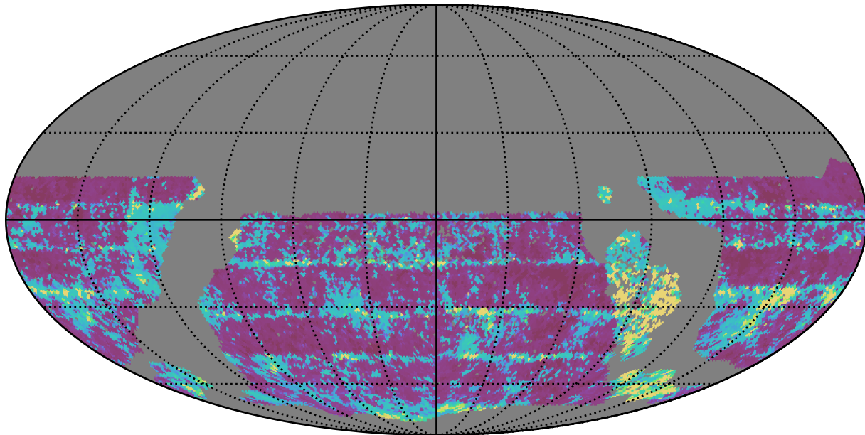
roman_v3.3_10yrs WFD z band: 20thPercentile Inter-Night Gap
