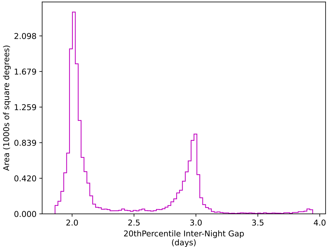
roman_v3.3_10yrs WFD z band: 20thPercentile Inter-Night Gap
