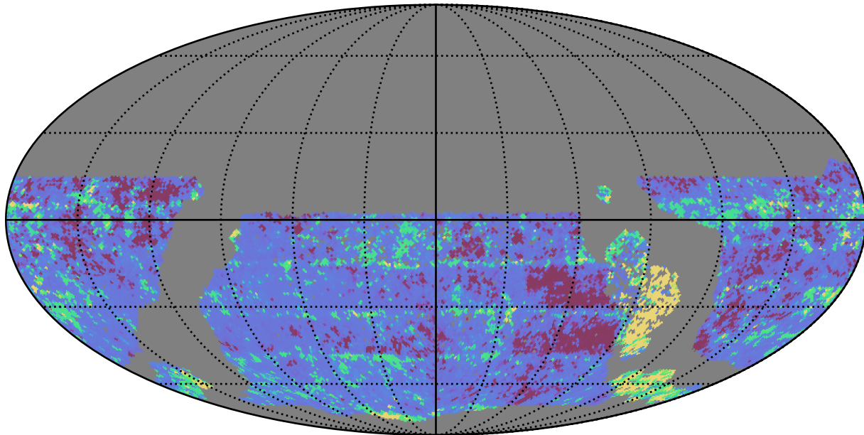
roman_v3.3_10yrs WFD y band: 20thPercentile Inter-Night Gap
