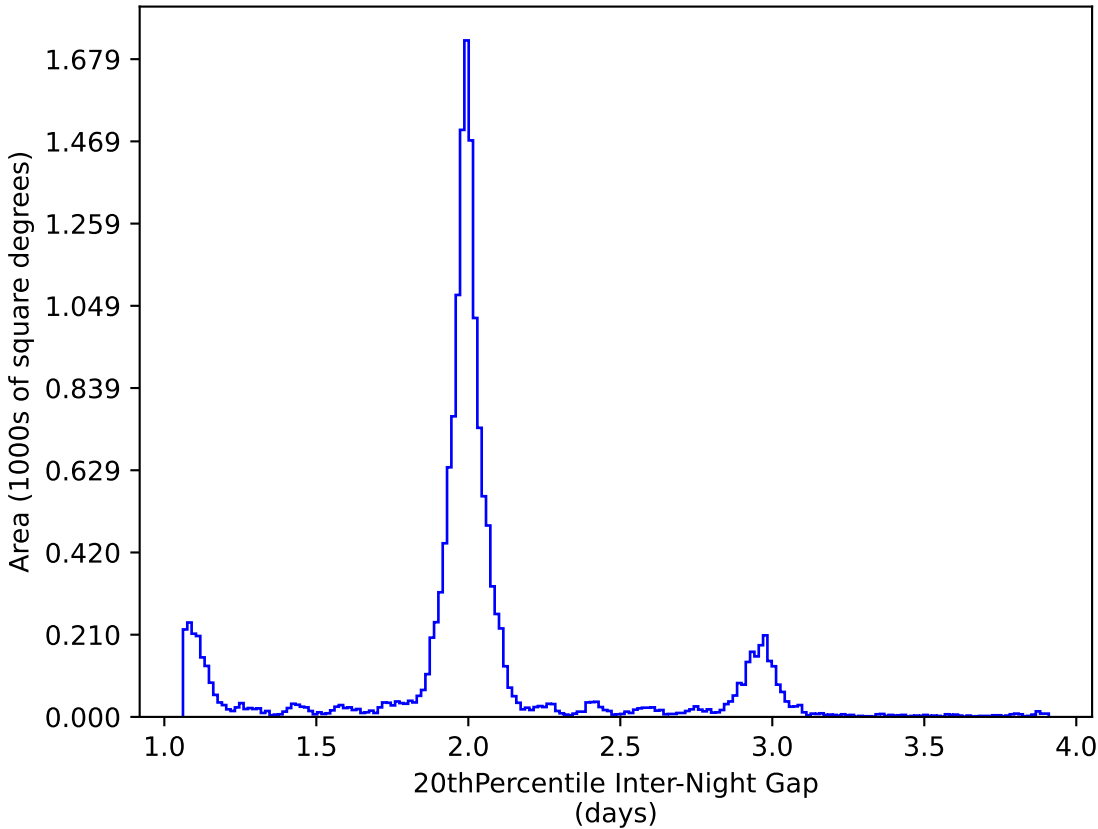
roman_v3.3_10yrs WFD y band: 20thPercentile Inter-Night Gap
