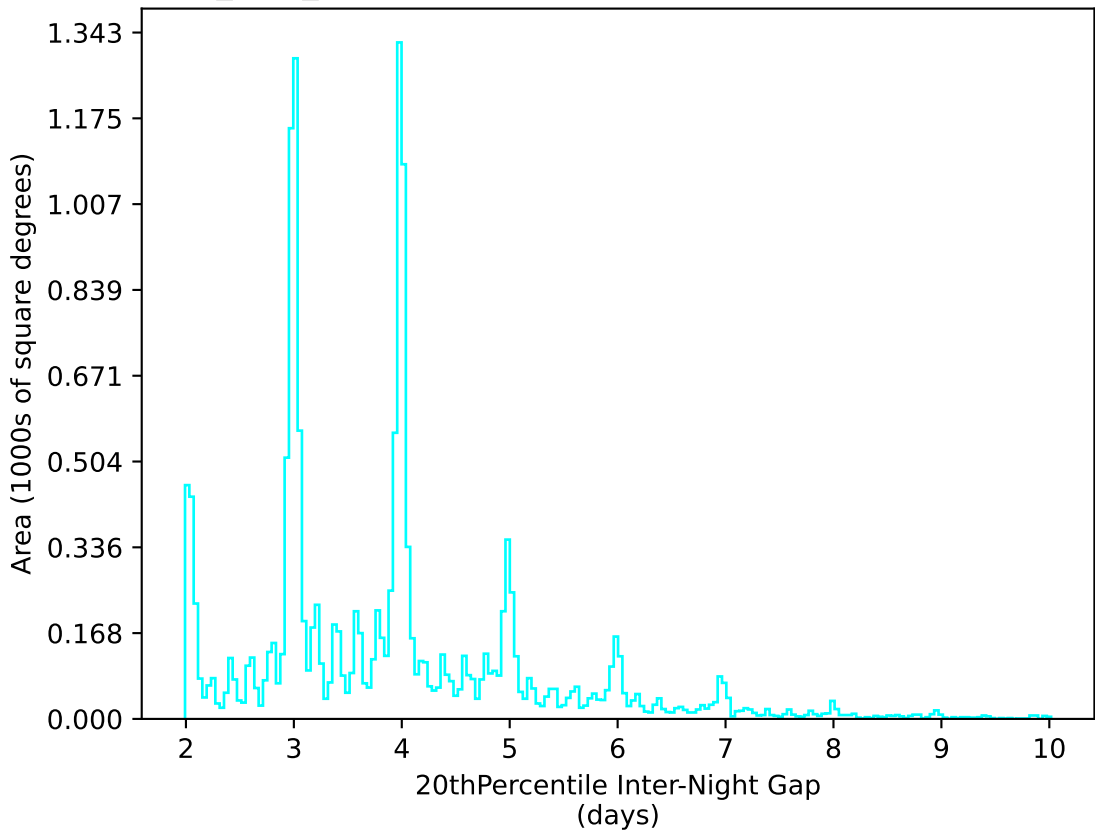
roman_v3.3_10yrs WFD u band: 20thPercentile Inter-Night Gap
