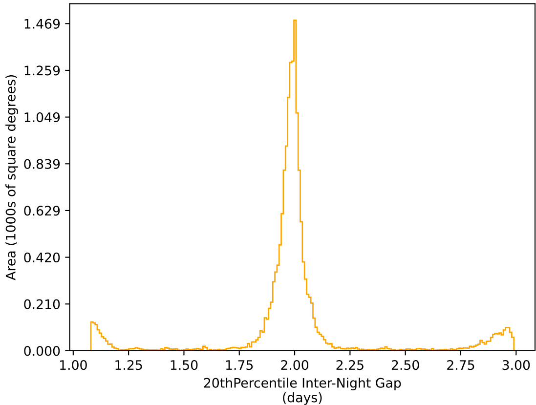
roman_v3.3_10yrs WFD r band: 20thPercentile Inter-Night Gap
