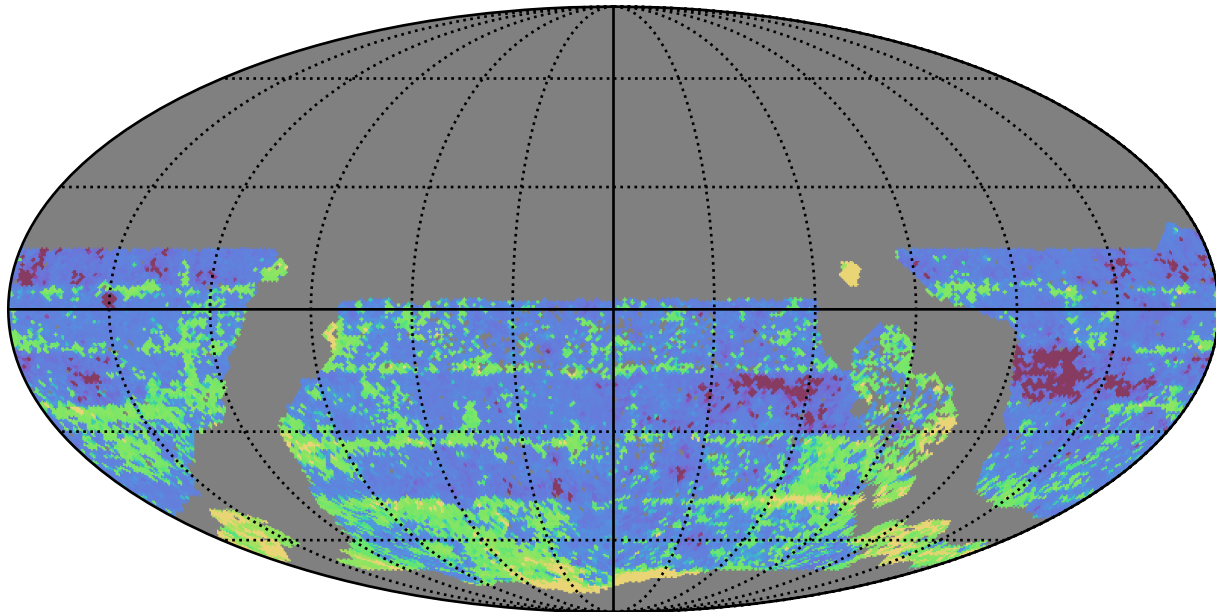
roman_v3.3_10yrs WFD i band: 20thPercentile Inter-Night Gap
